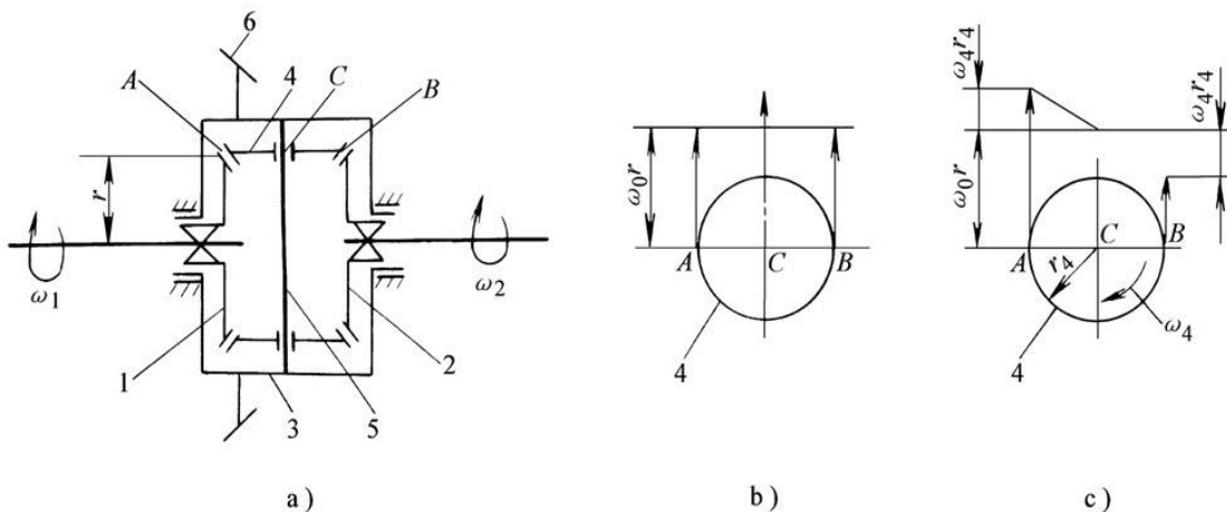
Fig. 2-4 Differential Principle
